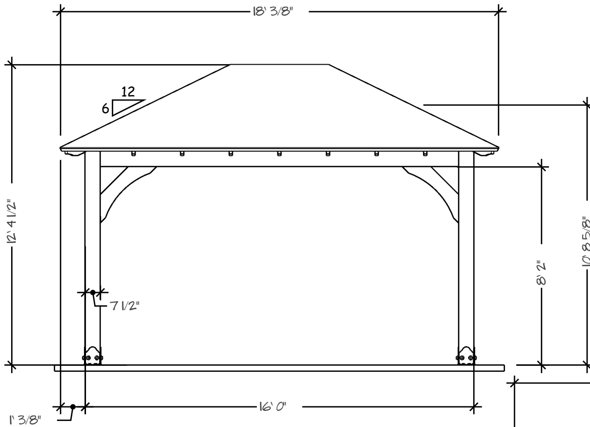
1 FRONT ELEVATION Scale: 1/4" : 1'
